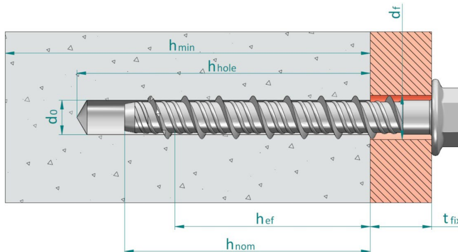
FIGURE 1—ANCHOR DIMENSIONS
